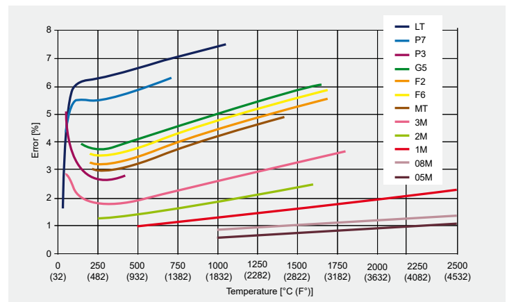
Measuring error in the case of emissivity wrongly adjusted by 10% as a function of the wavelength and object temperature (LT: 8–14 \mu\text{m} ; P7: 7.9 \mu\text{m} ; P3: 3.43 \mu\text{m} ; G5: 5 \mu\text{m} ; MT: 3.9 \mu\text{m} ; F2: 4.24 \mu\text{m} ; F6: 4.64 \mu\text{m} ; 3M: 2.3 \mu\text{m} ; 2M: 1.6 \mu\text{m} ; 1M: 1.0 \mu\text{m} ; 08M: 800nm; 05M: 525 nm).
