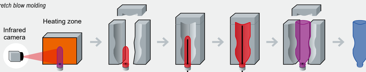
(Injection) stretch blow molding
