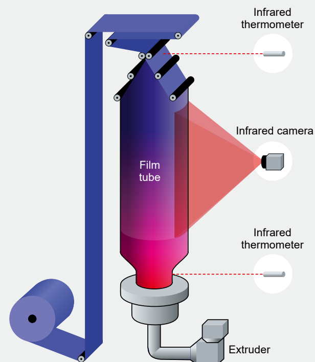
Extrusion blow molding of films
