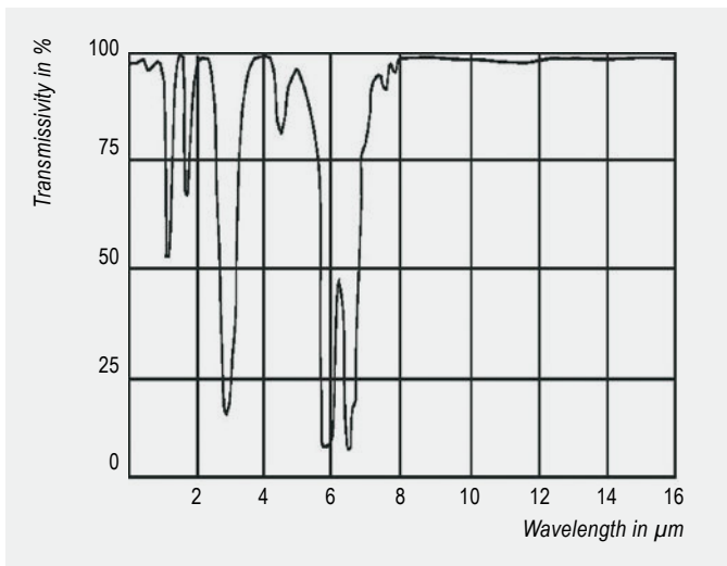
Spectral transmissivity of air (1 m, 32 °C (3.3 ft, 89.6 °F), 75 % r. F.)
